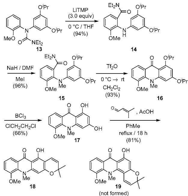
Scheme 4. Total Synthesis of Yukodine ( 17 ) and Junosidine ( 18 )
