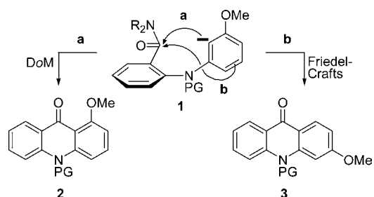
Scheme 1. Regiochemical Complementarity of Carbanion-Mediated and Lewis Acid-Catalyzed Cyclization Reactions
