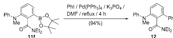
Scheme 3. Synthesis of Anthranilamide 12 by Suzuki–Miyaura Cross Coupling
